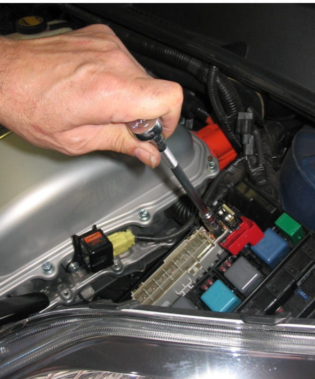
After turning the vehicle off, the technician disconnects the vehicle's auxiliary 12 V battery to ensure that the HV battery pack is mechanically isolated. The battery of this Toyota Prius can be disconnected from inside the main fuse/relay box.
